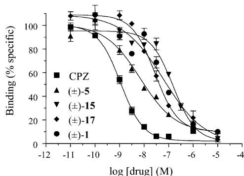
Figure 2. Representative competition binding curves for 5 (DNX) and its N -alkyl analogues at D 2 -like receptors in rat striatal membranes. The high-affinity, full agonist 1 (DHX) and the prototype antagonist chlorpromazine are included for comparison.
