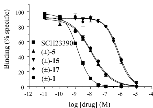
Figure 1. Representative competition binding curves for 5 (DNX) and its N -alkyl analogues at D 1 -like receptors in rat striatal membranes. The high-affinity, full agonist 1 (DHX) and the prototype antagonist SCH23390 are included for comparison.
