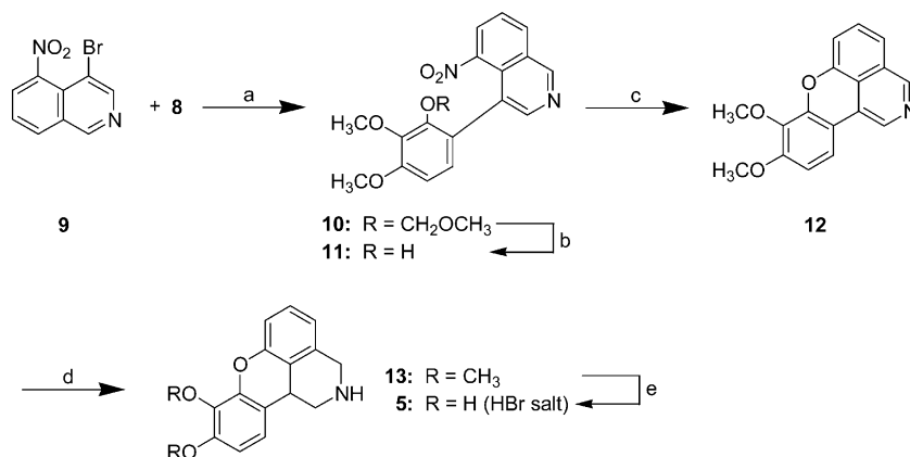
Scheme 2. (a) Pd(PPh 3 ) 4 , KOH, Bu 4 N + Cl − , H 2 O, DME, reflux; (b) TsOH·H 2 O, MeOH; (c) K 2 CO 3 , DMF, 80 °C; (d) PtO 2 , AcOH, HCl, H 2 ; (e) BBr 3 , CH 2 Cl 2 , −78 °C.
