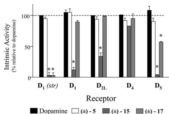
Figure 3. Maximal stimulation or inhibition of cAMP accumulation produced by 5 (DNX) and its N -alkyl analogues at D 1 -like and D 2 -like receptors. Compounds were evaluated in rat striatal tissue (D 1 -like) or in cells expressing the cloned receptors (monkey D 1 stably expressed in C-6 glioma, rat D 2L stably expressed in C-6 glioma, human D 4 stably expressed in CHO, or human D 5 transiently expressed in HEK 293). Emax values were determined from full dose-response curves. Data represent mean ± SEM from at least two experiments. * = significantly different from effects of dopamine ( P < 0.05 ).
