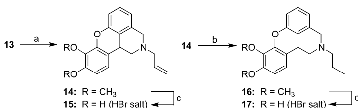
Scheme 3. (a) allyl bromide, acetone, K 2 CO 3 ; (b) H 2 , Pd-C, EtOH; (c) BBr 3 , CH 2 Cl 2 .
